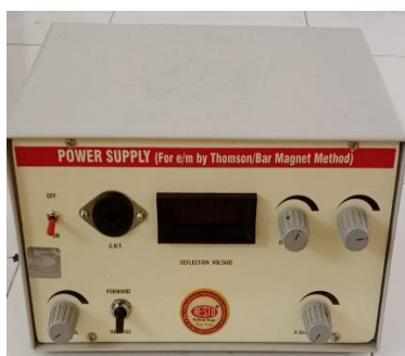
17. CRT Power Supply
